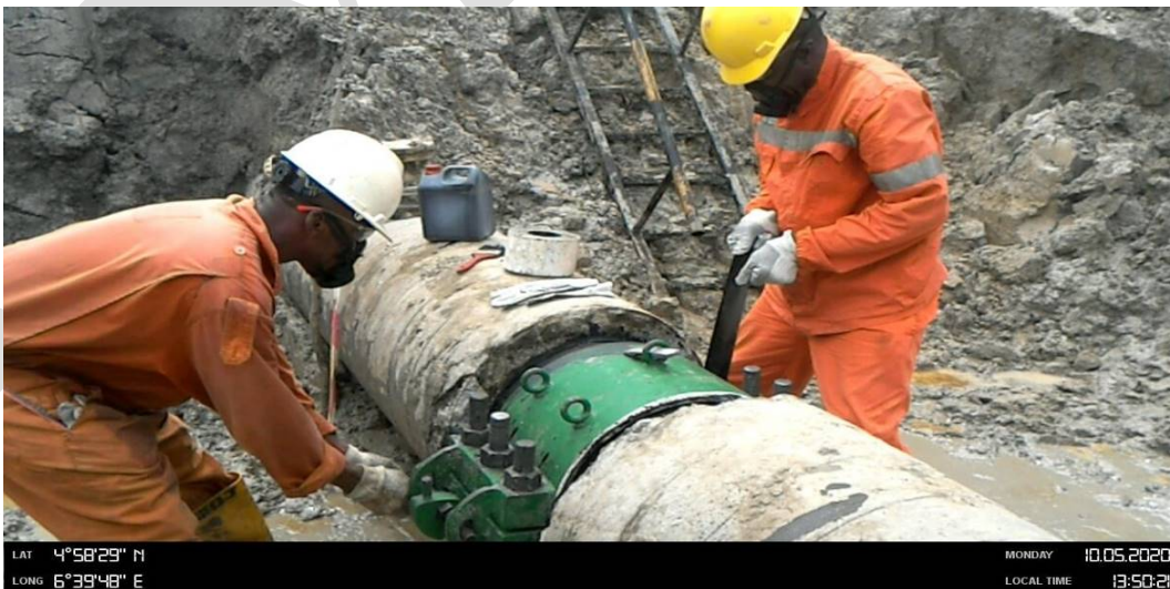
PERSONNEL WORKING INSIDE DITCH ON 20" KCTL AT OKOMA
